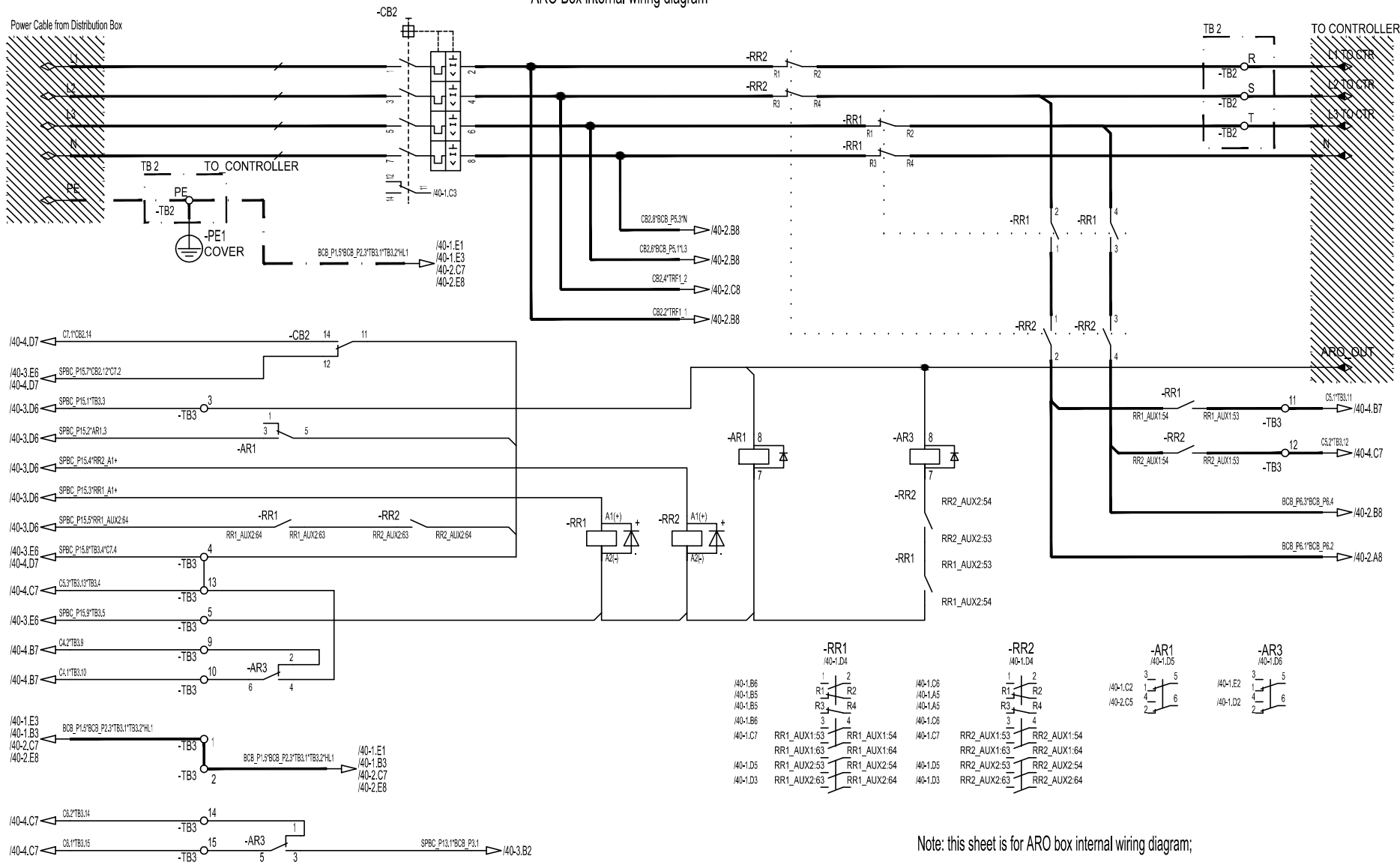
ARO Box internal wiring diagram
